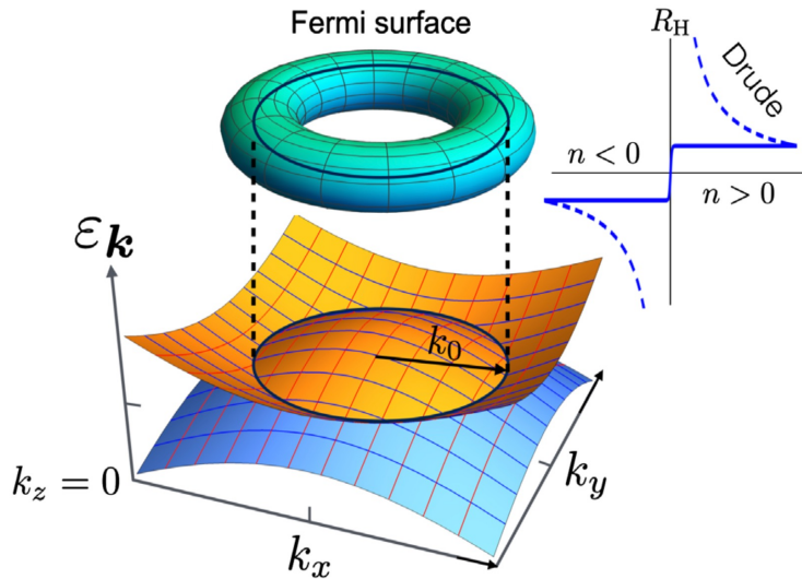
Deviation of Hall coefficient of nodal-line semimetals (solid blue) from Drude Relation (dashed blue)
