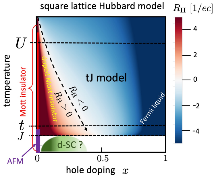
Hall coefficient map in Hubbard model
